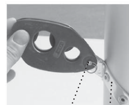
figure 66 | cleat, vang tang
